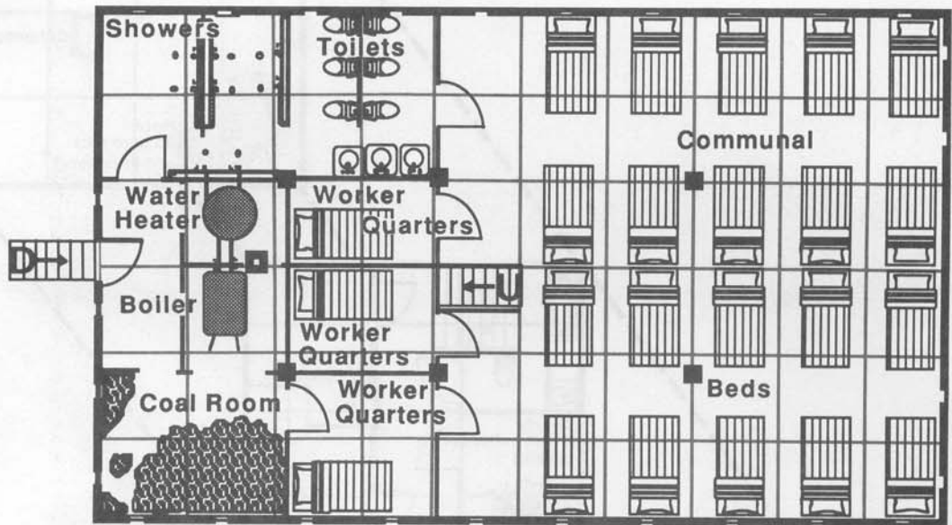
Basement (1.75 meters below ground level)
