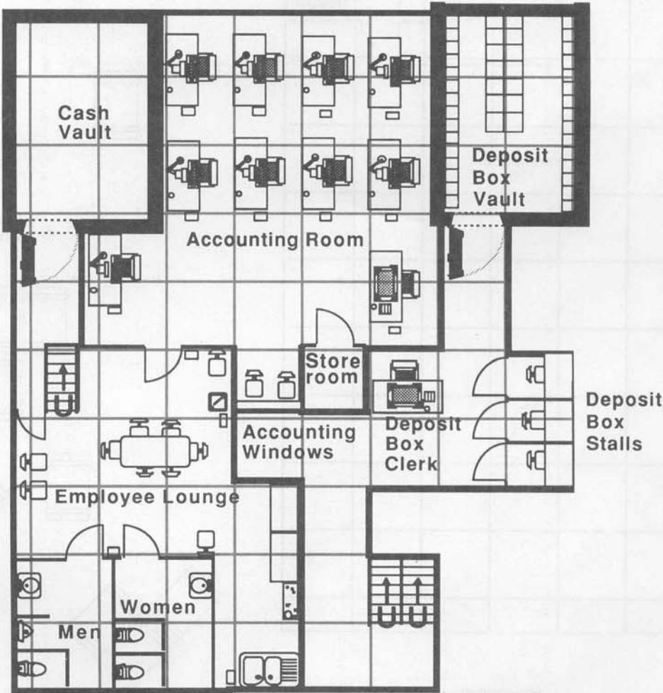
Basement (2 meters below ground level)
