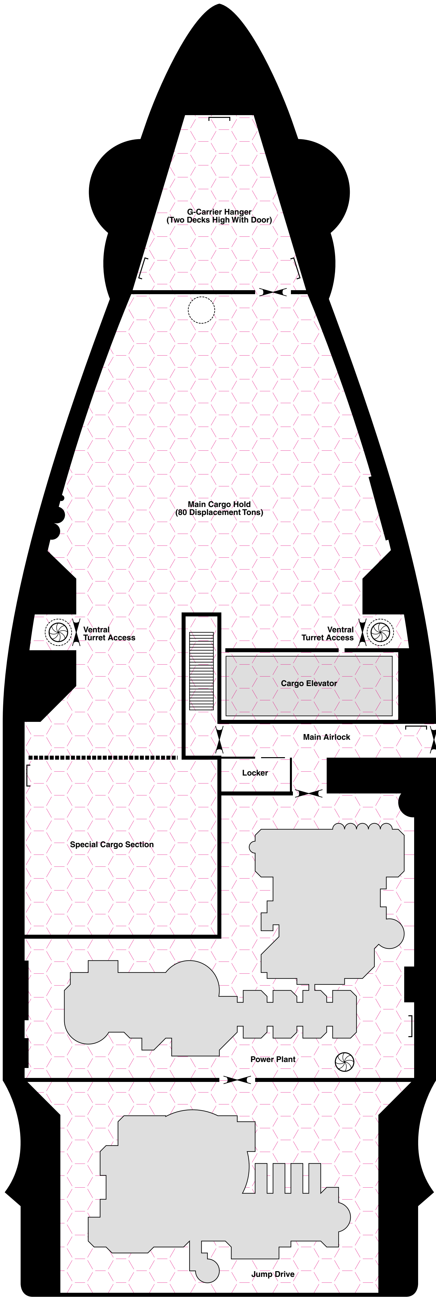
Deck 3
