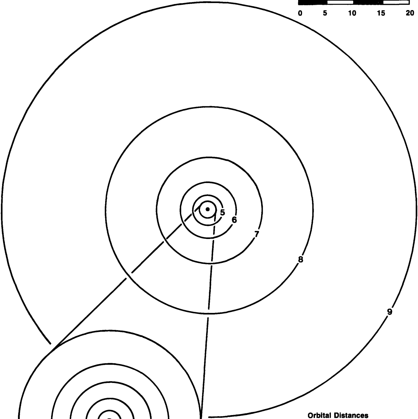
Orbital Distances
