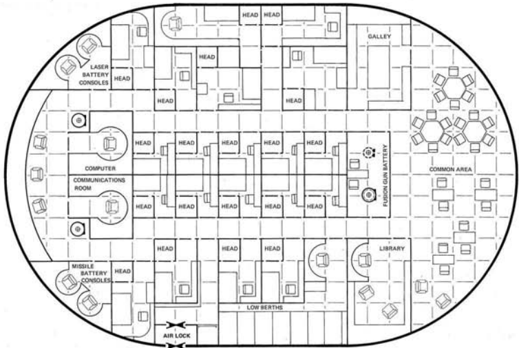
MAIN DECK
