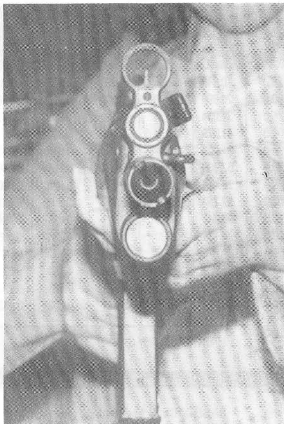
HK53 showing optional flashlight front grip with light control below muzzle. Pressure switch for light is just visible as the rectangular strip on the upper left side just above fingertips
