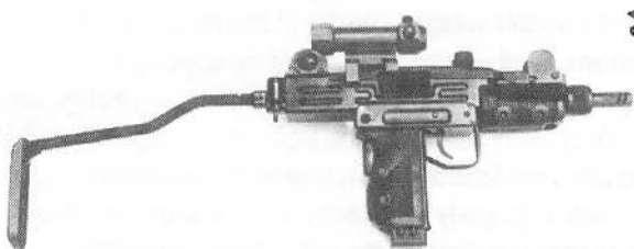
Mini UZI fitted with the Armson OEG sight, with 20 rd magazine
