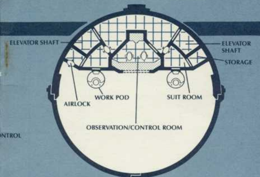
MAP 8. DOCK 2, MAINTENANCE DECK
