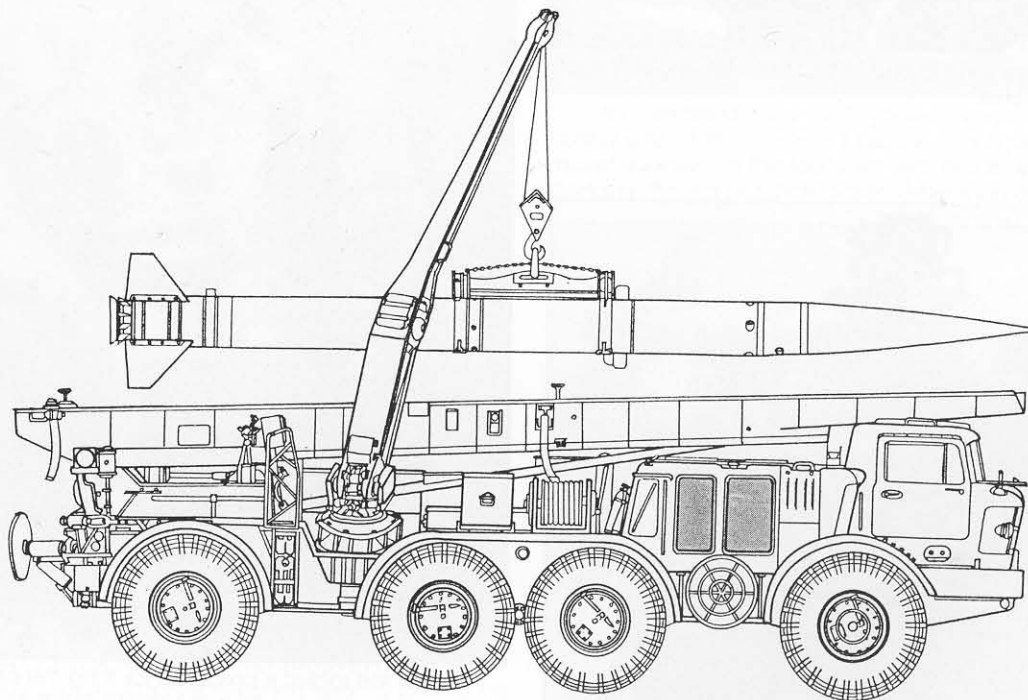
© S. Zaloga 1979 9P113 Luna-M Transporter-Erector-Launcher Vehicle (FROG-7)
