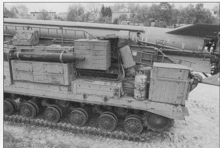
A view of the left rear of the 8U218 TEL showing the trunnion area and elevating mechanisms.
