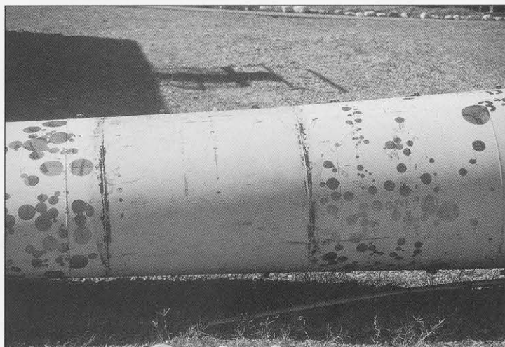
A detail shot of an Al-Husayn missile downed during the Gulf War by Patriots. The center section seen in this photo is one of two additional lengths of fuel tanks used to extend the Scud B missile for greater range. The dark circular pattern on the other sections resulted from the sand camouflage paint blistering from the heat during missile entry. The Al-Husayn was lengthened 1.3 meters (4' 3") compared to the normal Scud B.
