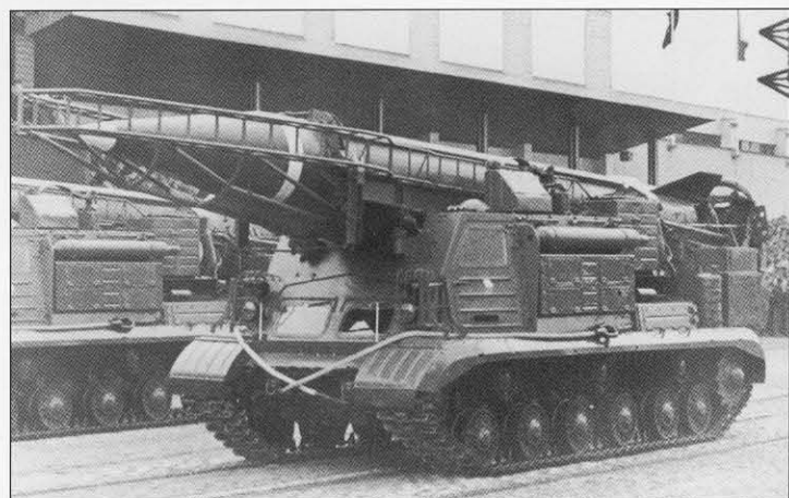
A pair of East German NVA 8U218 TEL (SS-1b Scud A) of the Lenkflugkörperbrigade "Otto Shwab", normally stationed at Hermsdorf with the 3.NVA-Armee. These vehicles remained in service into the 1970s, some of the last vehicles based on the ISU-152 assault gun to survive so long in service.
