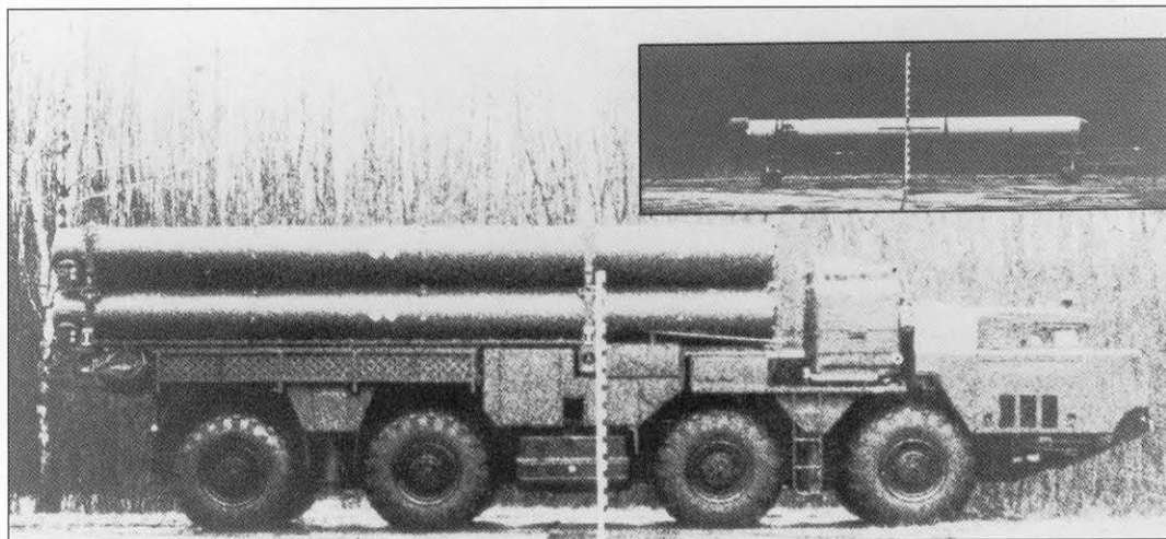
The 3P51M Rubezh-A coastal anti-ship missile launcher is based on the MAZ-7910 truck, very similar to the 9P117 used with the Scud B except for the absence of an auxiliary cab on the right side.
