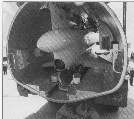
A view inside the launch tube shows the Tu-143 drone. A new version of the drone, the Tu-300, can be used as a UCAV (uninhabited combat air vehicle) to deliver cluster bombs against targets and then return back to base.
