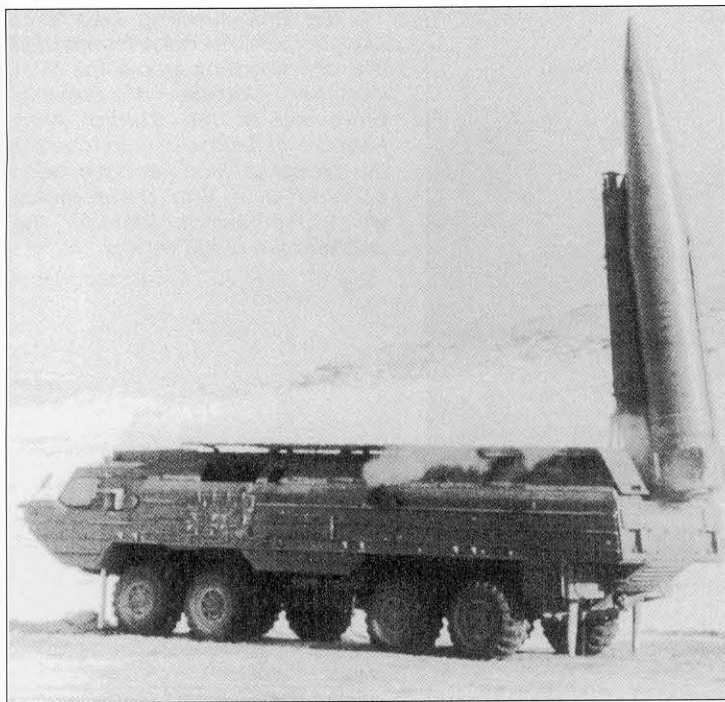
The Oka (SS-23 Spider) was developed as a replacement for the 9K72 Elbrus (SS-1c Scud B). It entered service in small numbers after 1986, but soon afterwards was withdrawn and dismantled due to the range restrictions of the INF Treaty. This is the Oka's 9P71 launcher vehicle, based on the BAZ-6944. It resembles an enlarged 9P129 from the Tochka system since they were both designed by the same organization.
