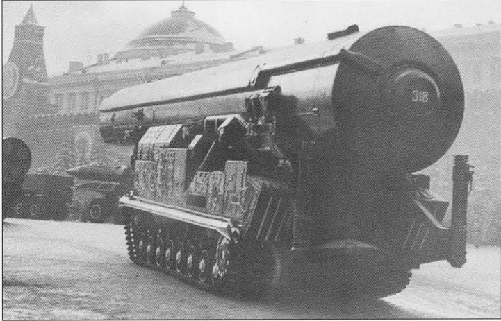
A rear view of the RT-20P's Obiekt 821 TEL showing the enormous stabilizing arms used to lock down the chassis during launch.
