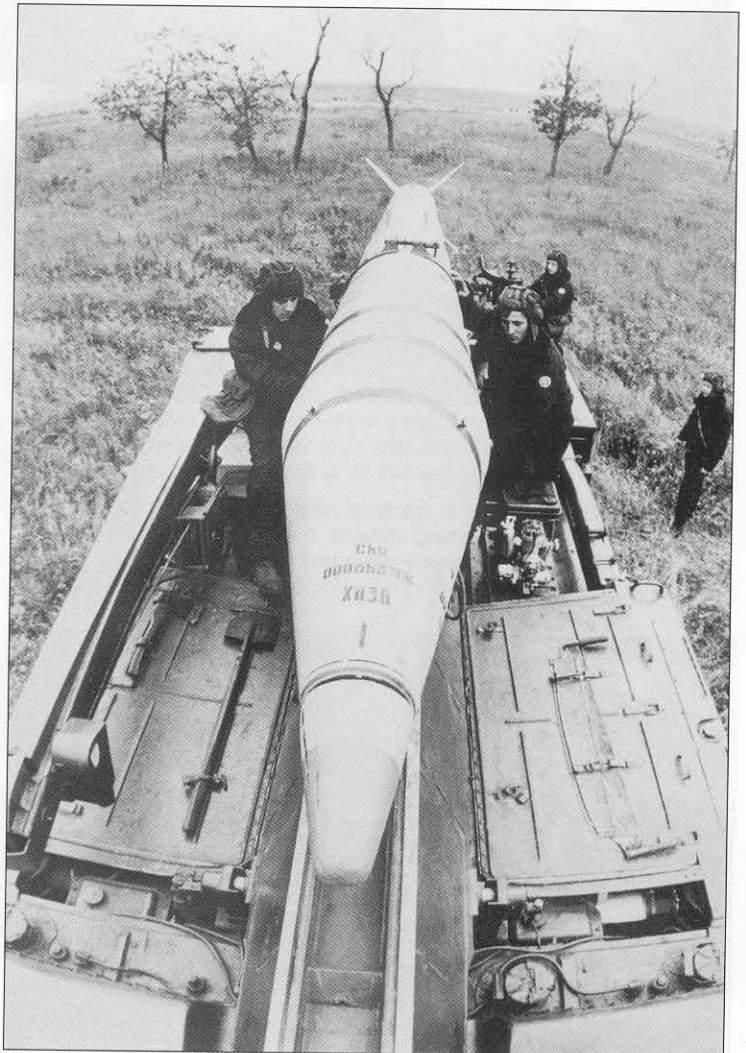
An interesting close-up of a Luna-M rocket warhead. The R-70 rocket is also known by its industrial index number 9M21. The 9M21 rocket comes in four combat types: the 9M21F with a 9N18F HE-Frag warhead; the 9M21E with the 9N18E submunitions warhead; the 9M21B with the AA22 nuclear warhead; and the 9M21 Kh with a chemical warhead filled with VX agent. Besides the tactical rockets, crews often use the PV-65, which is a training round.
