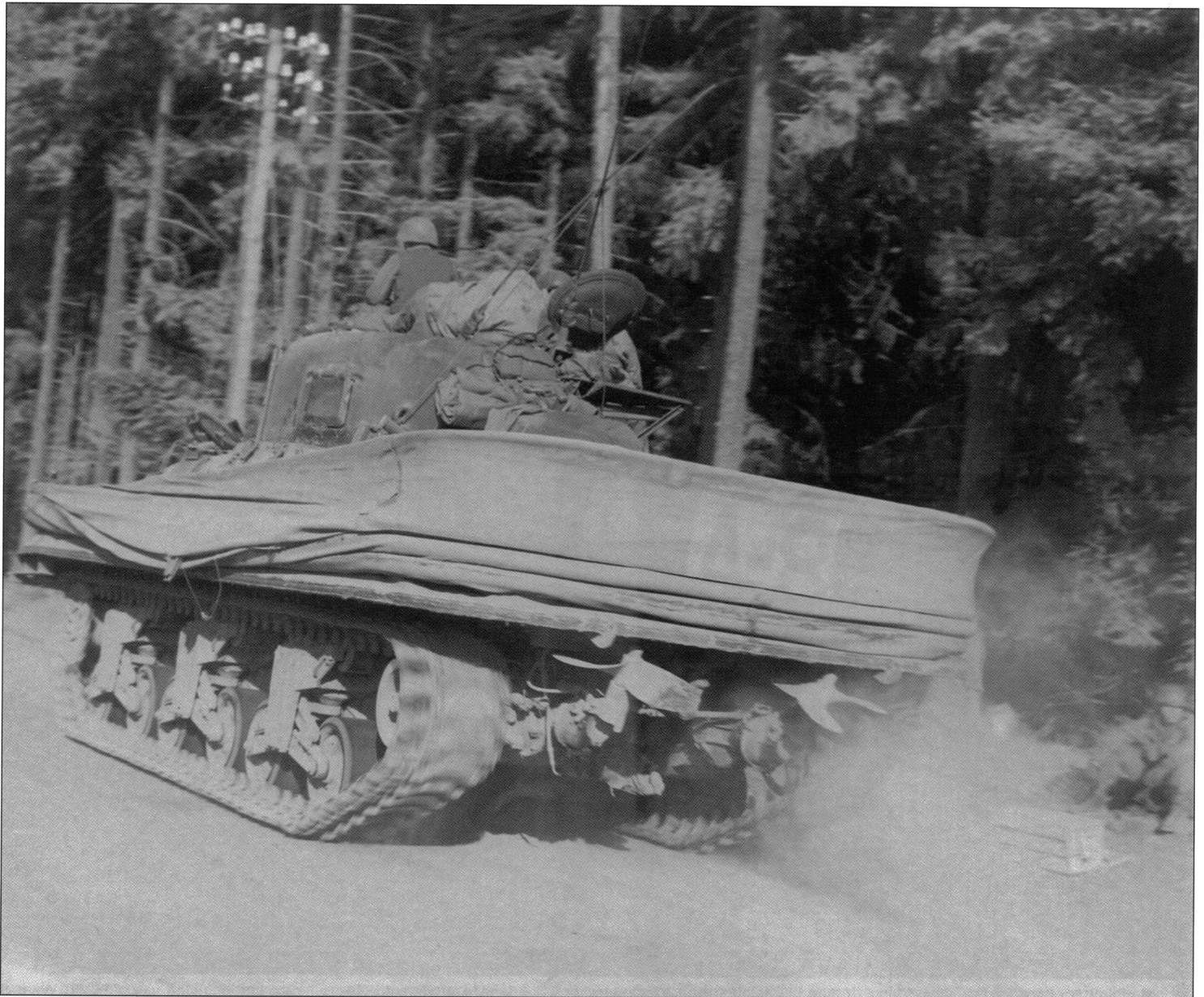
This is a very good view of a fully equipped Duplex Drive M4A1 medium tank of Patton's 3rd Army near Braunschweig, Germany on 24 March 1945 after the Rhine crossings. This shows the screen folded down, and the propellers in the retracted position. (US Army)
