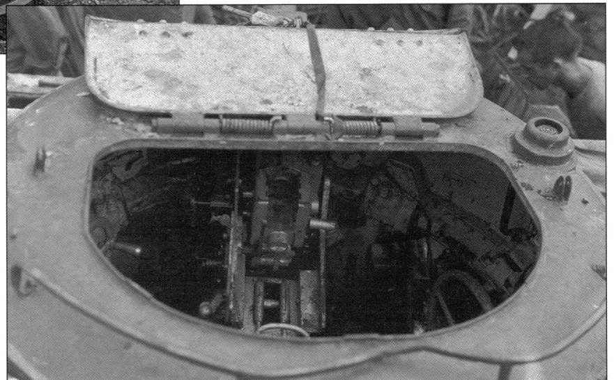
A detail view looking into the hatch of a Type 2 Ka-mi, and showing the gun breech of the 37mm gun. (US Army)
