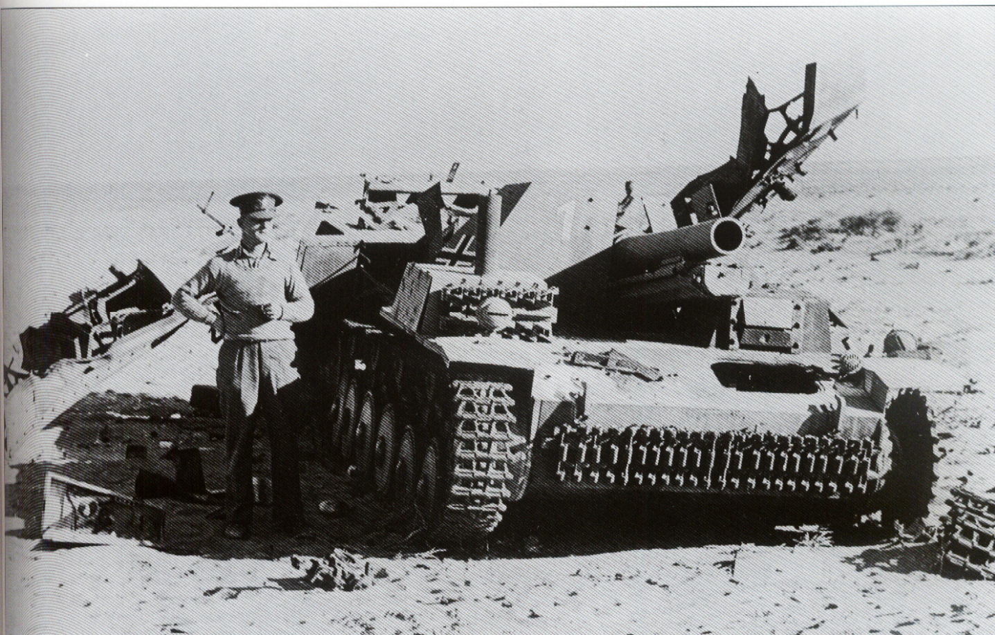
A 15cm s.I.G.33 B Sfl. from s.I.G.Kp.(mot.S) 707 or 708 that has been destroyed by an anti-tank round that has set off the ammunition stored in the back of the vehicle. Twelve of these self-propelled guns were sent to Libya, six in February 1942 and the remainder in April. The weight of the gun overloaded the chassis and they suffered from many automotive problems during their short combat history. After the battle of El Alamein, the British reported capturing six in various states of repair. German reports indicate that all were lost by December 2, 1942.
