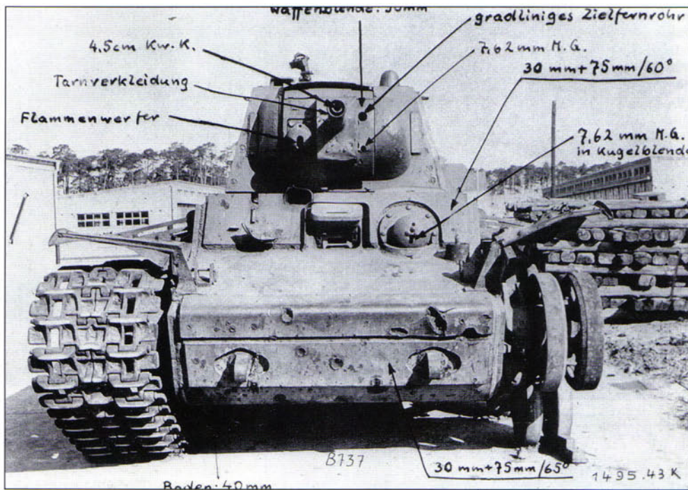
This German intelligence photo shows a captured KV-8 flamethrower tank. This frontal view clearly shows the 45mm gun within a thick sheet metal barrel. The flamethrower housing can be seen low to the left of this.
