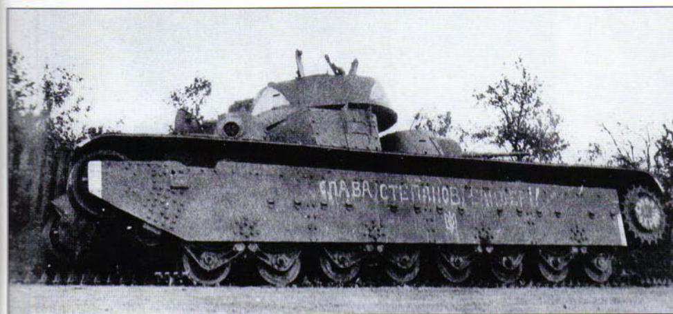
A total of 48 T-35 heavy tanks were operational with the Red Army at the beginning of the war on 22 June 1941 with the 67th and 68th Tank Regiments of the 34th Tank Division, 8th Mechanized Corps in Ukraine. Of these, only 5 were lost in combat, the remainder were abandoned due to mechanical breakdowns. This is the standard T-35 Model 1935 identifiable by its vertical turret sides. (James Crow)
