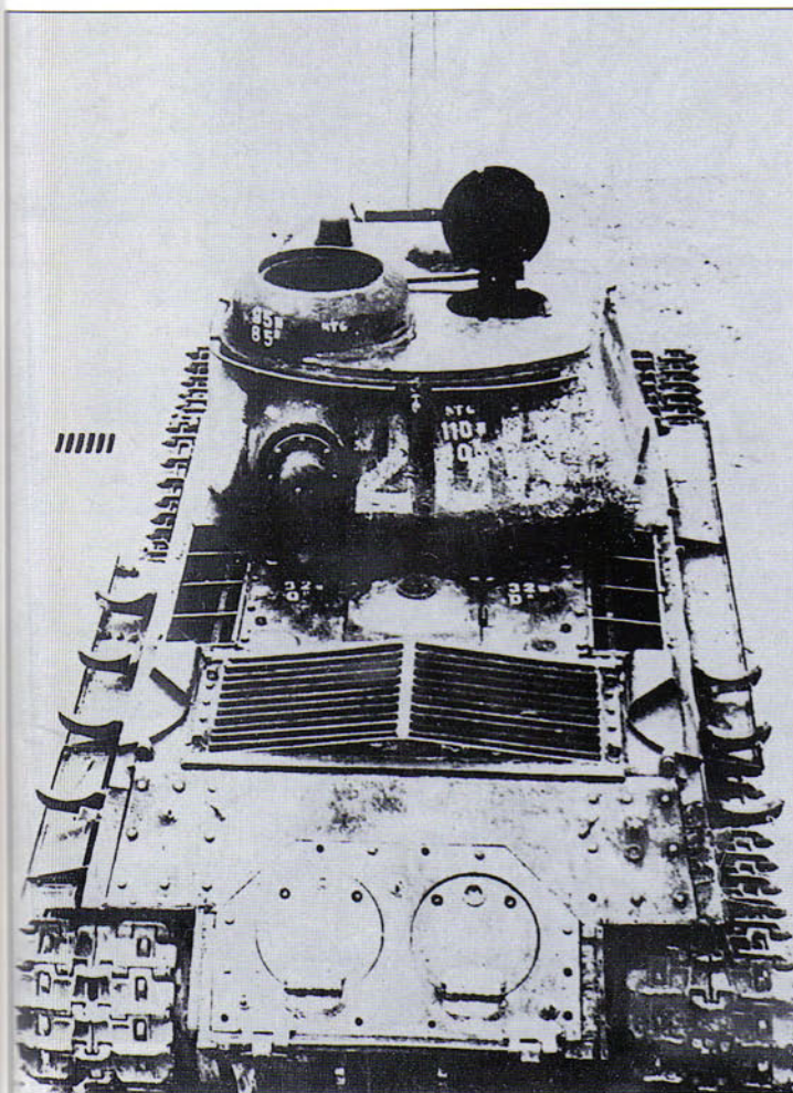
A rear view of the early IS-2 captured by the Germans. There are several interesting details evident in this view such as the lack of a rear travel lock, and the KV-85 style of wrap-around hand-holds on the turret.
