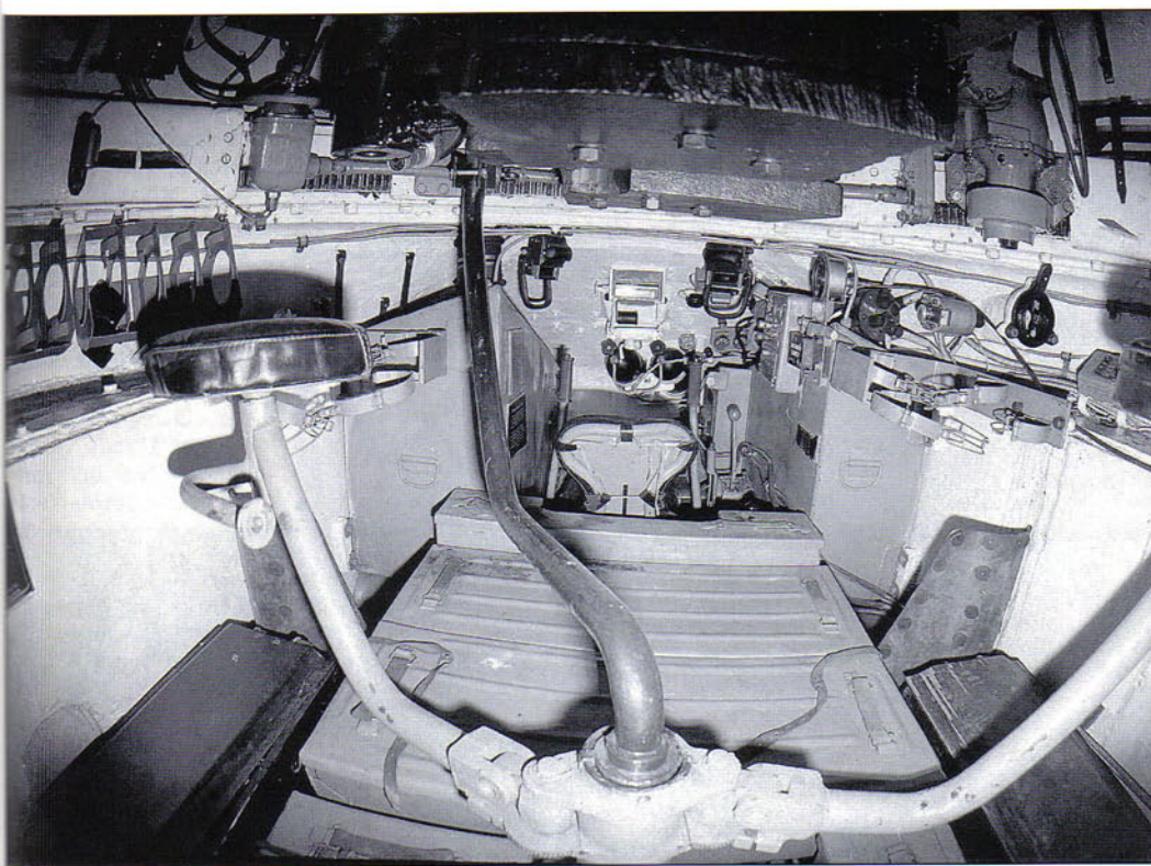
A view from below the gun breech towards the driver's station. The piping in the center of the hull is for the gunner's seat on the left, the turret electrical conduit in the center and the loader's seat on the right. The driver's compartment is in the center of the vehicle and is flanked by two fuel tanks. The floor is made up of metal ammunition lockers for the reserve ammunition supply. The IS-2 carried only 28 rounds of ammunition, 12 in the ready reserve, and the remainder in the hull.
