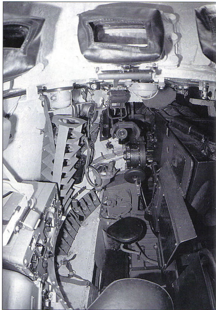
The IS-2 enjoyed a substantially better interior design than the KV series with a much more practical turret layout. This view of an IS-2M currently preserved at Duxford shows a view from the commander's station on the left hand side forward towards the driver's station. In the IS-2, the radio was near the commander rather than in the hull to facilitate communication.
