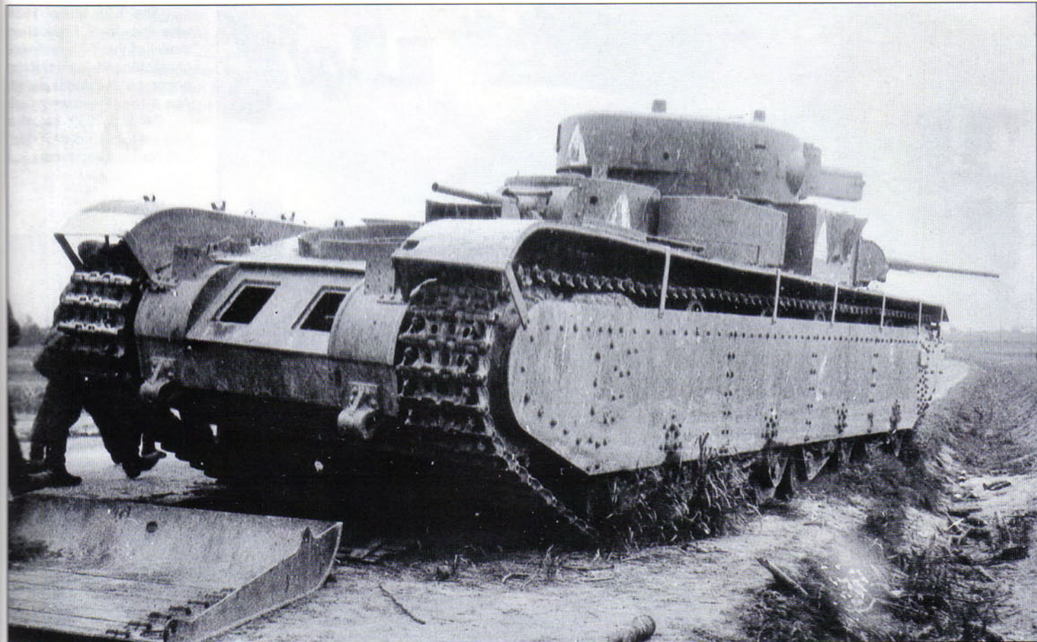
A total of 48 T-35 heavy tanks were operational with the Red Army at the beginning of the war on 22 June 1941 with the 67th and 68th Tank Regiments of the 34th Tank Division, 8th Mechanized Corps in Ukraine. Of these, only 5 were lost in combat, the remainder were abandoned due to mechanical breakdowns. This is the standard T-35 Model 1935 identifiable by its vertical turret sides. (James Crow)
