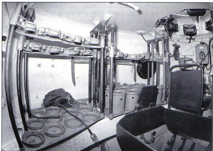
The ready ammunition for the IS-2 was kept in the rear right hand side of the turret bustle behind the loader. The 122mm gun used split case ammunition with the propellant cases to the outside of the racks and the projectiles towards in the inside.
