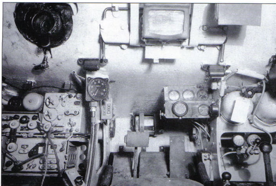
A view of the driver's station in the KV. The driver sat in the center of the hull, and his controls are evident in this view. To the left was the station for the radio-operator/hull machine gunner. The socket for the front DT machine gun is evident in this view, although the machine gun is not fitted. (US National Archives)
