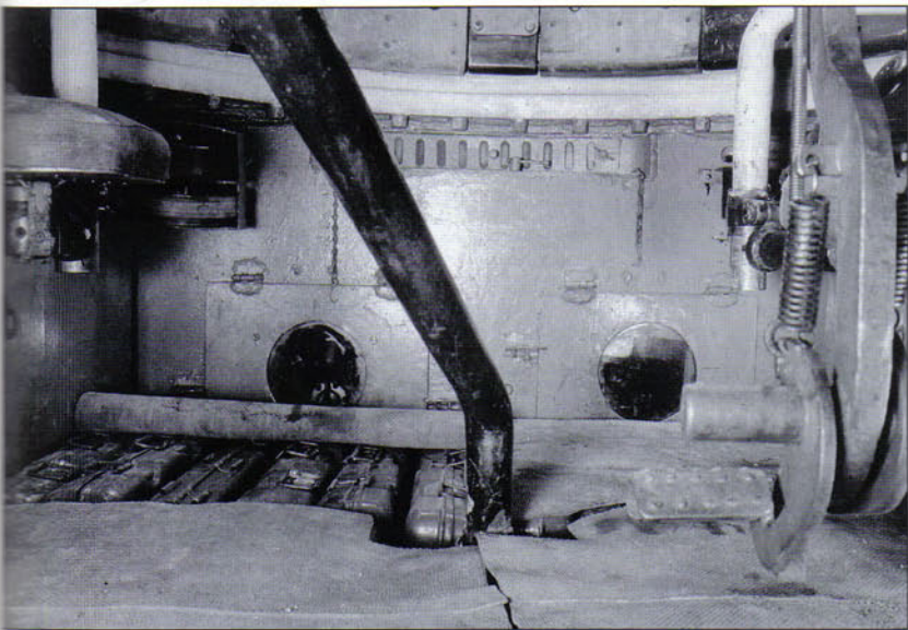
A view looking back from the driver's station towards the rear firewall at the back of the fighting compartment. The most striking detail in this photo is that Soviet tanks did not have turret baskets. The large pipe in the center of the photo was a conduit for electrical lines running up into the turret. The device at the right is the gunner's firing pedals, while the loader's seat can be seen at the left. The floor consisted of metal stowage boxes containing 76.2mm tank gun ammunition. These containers were covered by rubber floor mats, one of which has been pulled away to the left to show the ammunition containers. (US National Archives)
