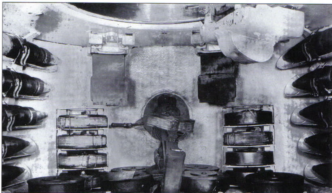
A view of the rear of the turret of the KV-1 Model 1941. At the center is a DT 7.62mm machine gun. The third crewman in the turret has the responsibility for operating this machine gun, intended to provide defense against enemy infantry. This layout was archaic, and due to crew shortages in 1942-43, this position was often left unfilled. The main gun ready ammunition racks can be seen on either side of the turret, as well as the drum magazines for the DT machine gun.
