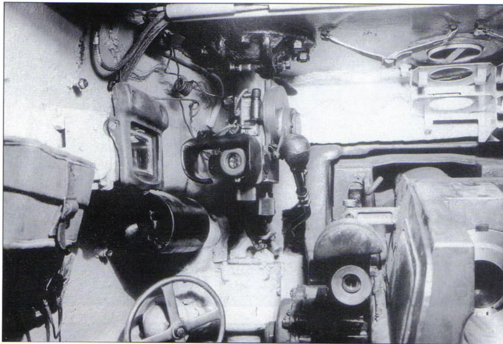
A close-up of the gunner's station in the KV-1 Model 1941. The gunner had two sets of optics to aim the gun, either the TMFD telescopic sight adjacent to the gun breech, or the PTK periscopic sight mounted in the roof. The large wheel in the lower left of the photo is for manually traversing the turret. (US Army Ordnance Museum, APG)
