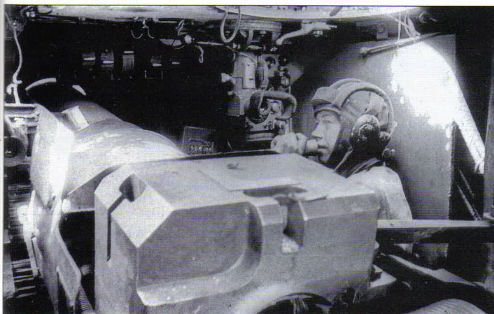
The interior of the SU-152 was very cramped, as can be seen from this shot inside a vehicle on 6 July 1943 during the battle of Kursk. Although intended for direct fire support, during the Kursk battle the SU-152 was used occasionally as a tank destroyer since it was one of the few Soviet armored vehicles with a gun large enough to penetrate the new Tiger, Panther and Elephant. Its success in this role led to its nickname "Zvierboi"- Animal Hunter. (P. Troshkin)
