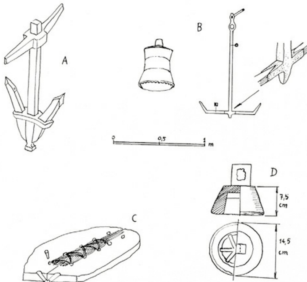
Elements of late antique ships: A) wooden anchor with lead log and ferrule; B) iron anchor and copper pitcher from the Cervia boat; C) sewings of the planks of the Cervia boat, fourth century AD; D) lead sounding of the Cervia boat. (Drawing by Andrea Salimbeti ex Bonino)
