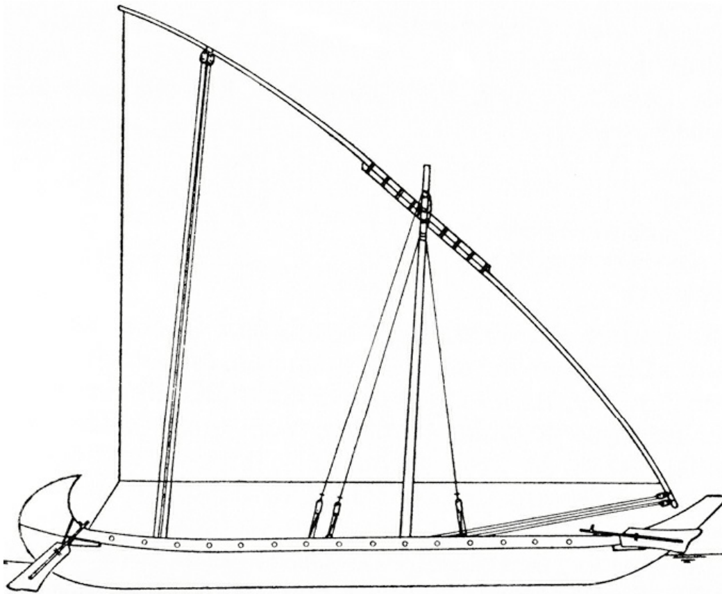
Reconstruction of a ship for marines' transport, fifth century AD. (Drawing by Andrea Salimbeti ex Viereck)
