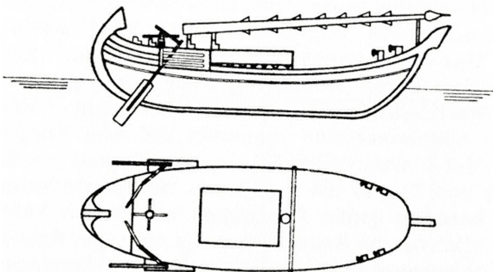
Reconstruction of a navis oraria , fifth century AD. (Drawing by Andrea Salimbeti ex Viereck)
