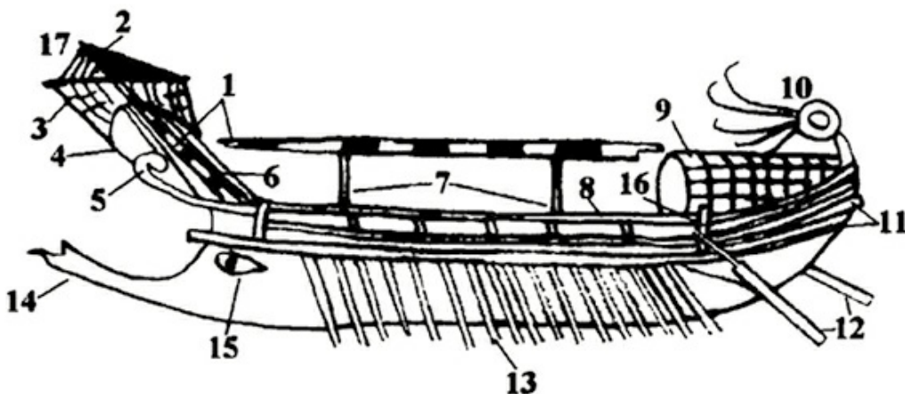
Roman ponto , Classis Nova Lybica , c. 200–20 AD. The bow shape is concave, the stern shape is convex, square rig. (Mosaic from the baths at Themetra near Hadrumetum, Carthage, Tunisi, Bardo drawing by Andrea Salimbeti ex Royal)
