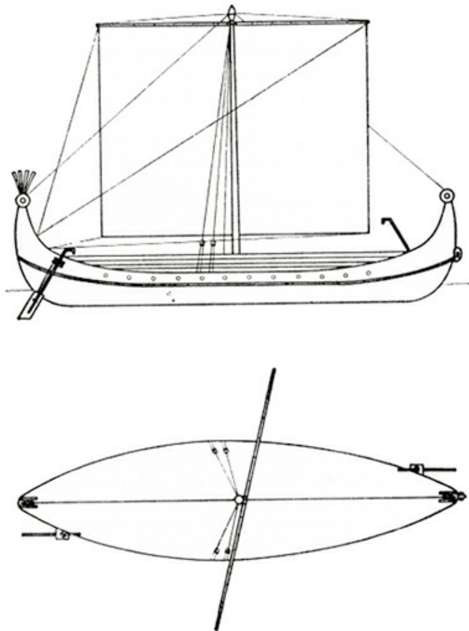
Reconstruction of a camara , fourth century AD. (Drawing by Andrea Salimbeti ex Viereck)
