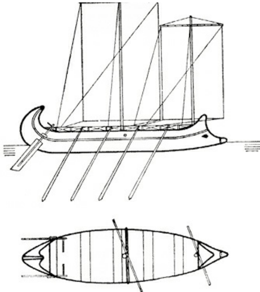
Reconstruction of a navis lusoria , fourth century AD. (Drawing by Andrea Salimbeti ex Viereck)
