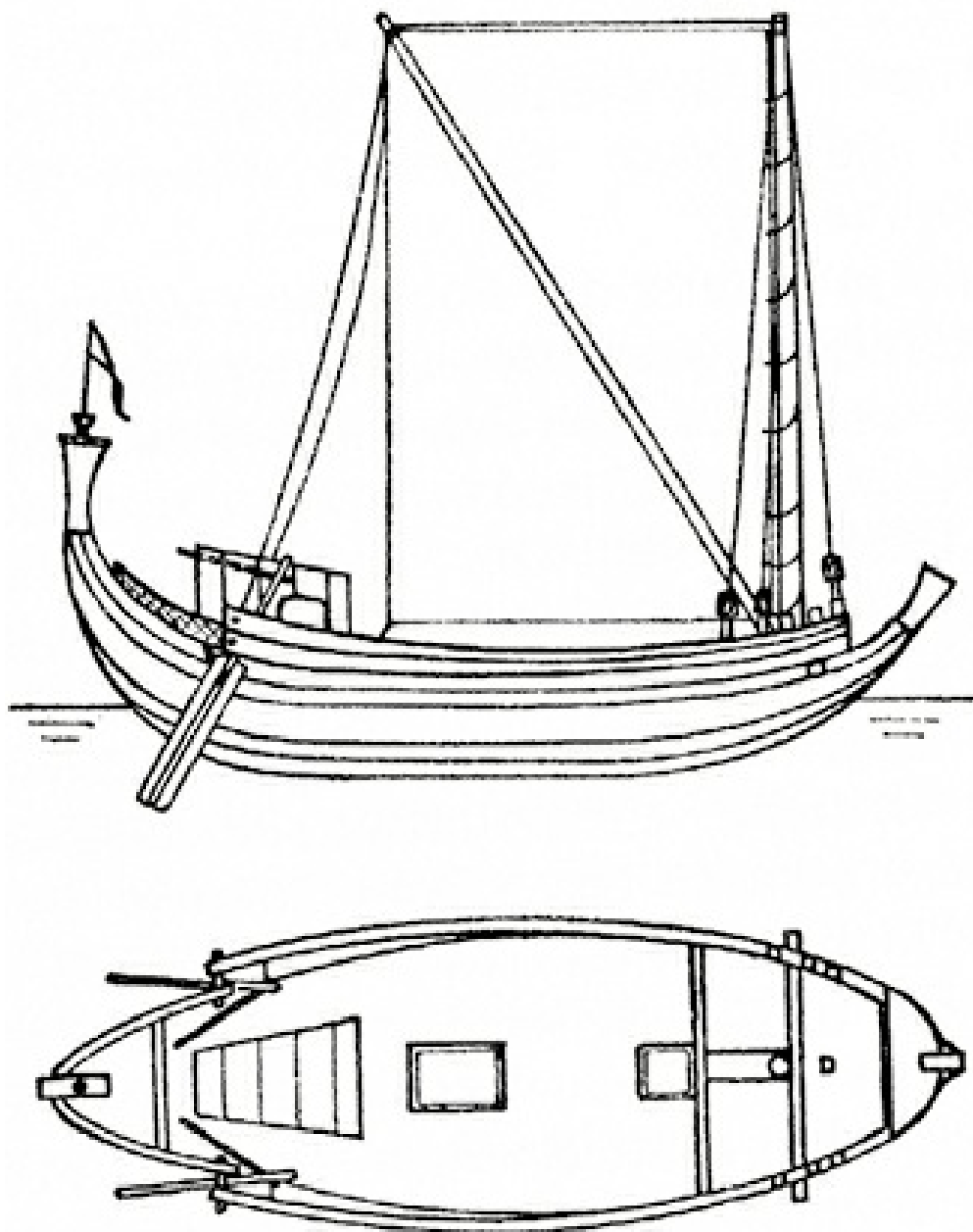
Reconstruction of a navis oraria , 2nd–3rd century. (Drawing by Andrea Salimbeti ex Viereck)
