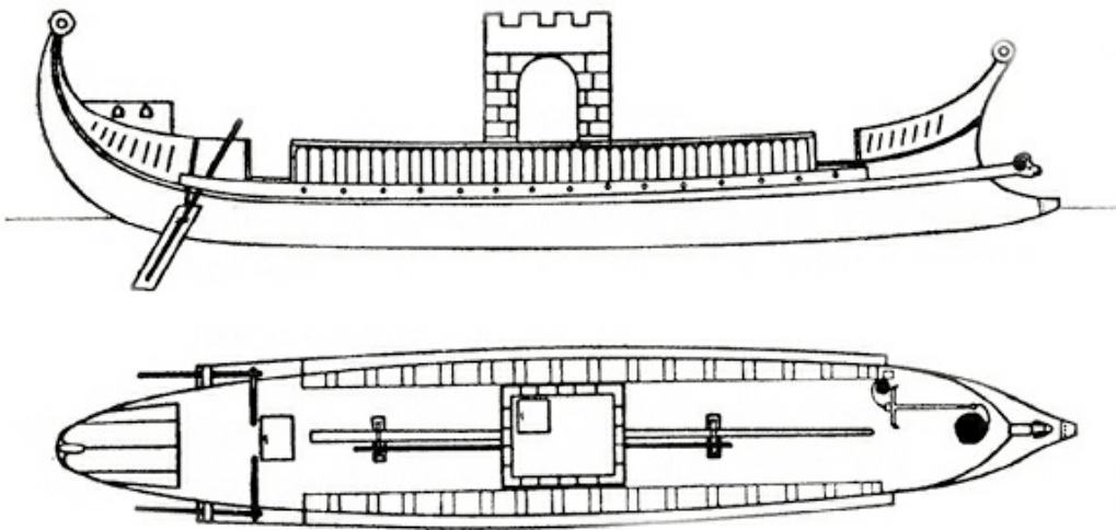
Reconstruction of a triakonteris of Constantine the Great, 324 AD. (Drawing by Andrea Salimbeti ex Viereck)
