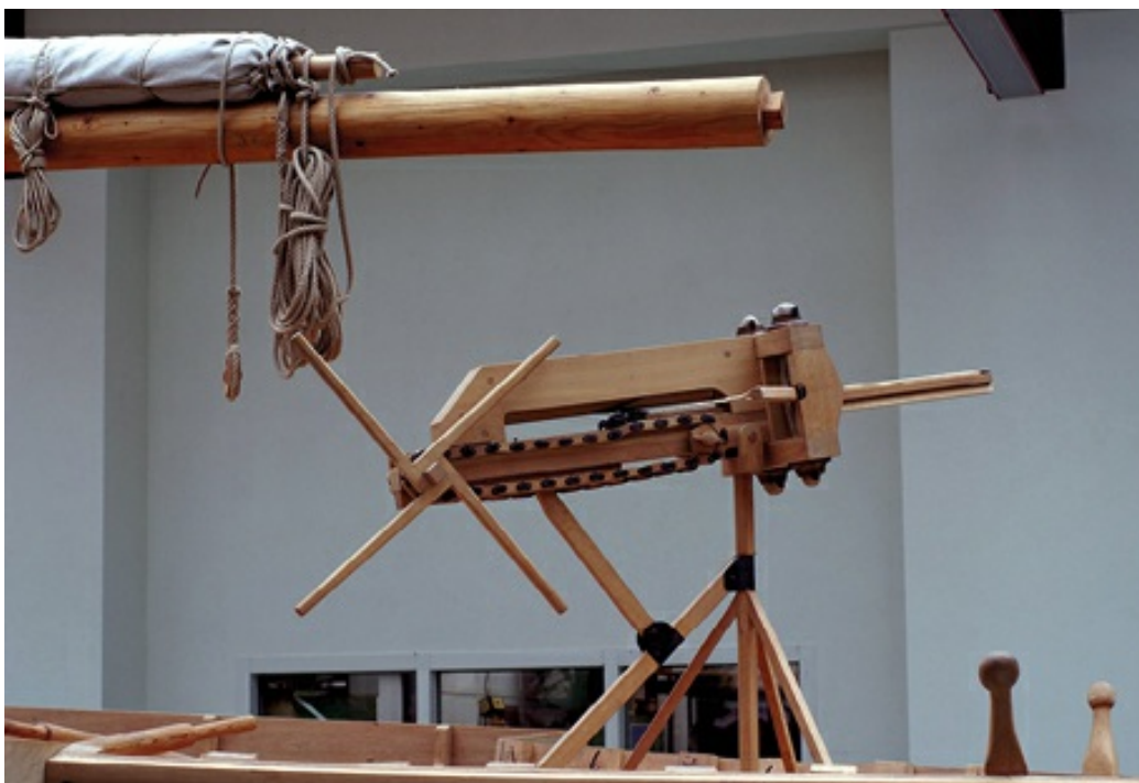
Catapult mounted on a warship, fourth century AD. (Reconstruction by the Museum für antike Schifffahrt in Mainz, Mainz, photo courtesy of the museum)
