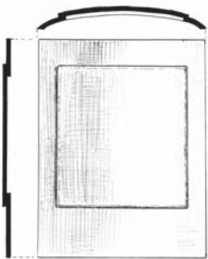
Sample of one of the 18 iron plates probably once used in elephant armour, found at Taxila and dating from the 1st century BC to 1st century AD. The plate is 25.4 × 21.6cm (10 × 8.5in). Every plate is slightly bent along its vertical axis and has a projecting central part, which was meant to enhance the protective effect: at a blow the plates spring, weakening the penetration. (After J. Marshall)
