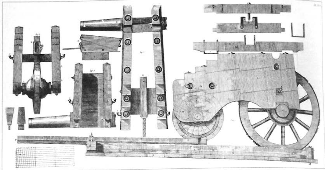
Plan of the profile, top and rear of a Gribauval garrison carriage for a 16-pdr and its platform. (Print after de Scheel)
