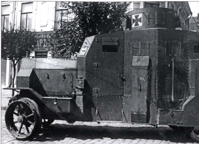
German tanks were never deployed on the Russian front, but there was a proliferation of armored car units there in 1918 for occupation duty. This is an Erhardt E-V/4 1917 on patrol in Rostov in Russia in 1918. (NARA)
