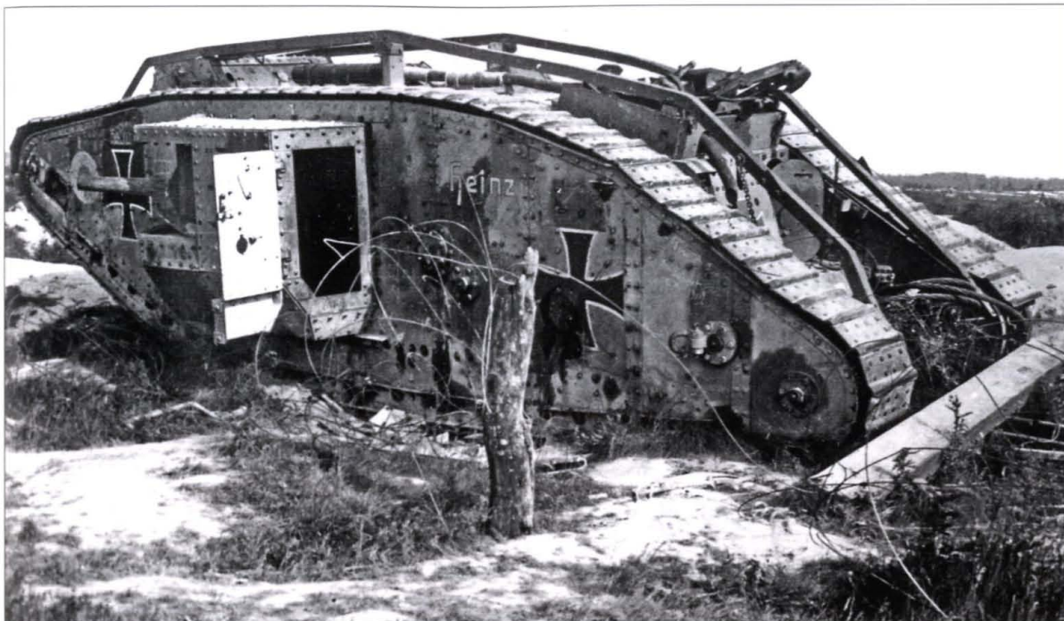
"Heinz," Panzer 207, the No.4 tank of Abteilung 14, was lost in action during the fighting near Fort de la Pompelle on June 1, 1918. (Patton Museum)
