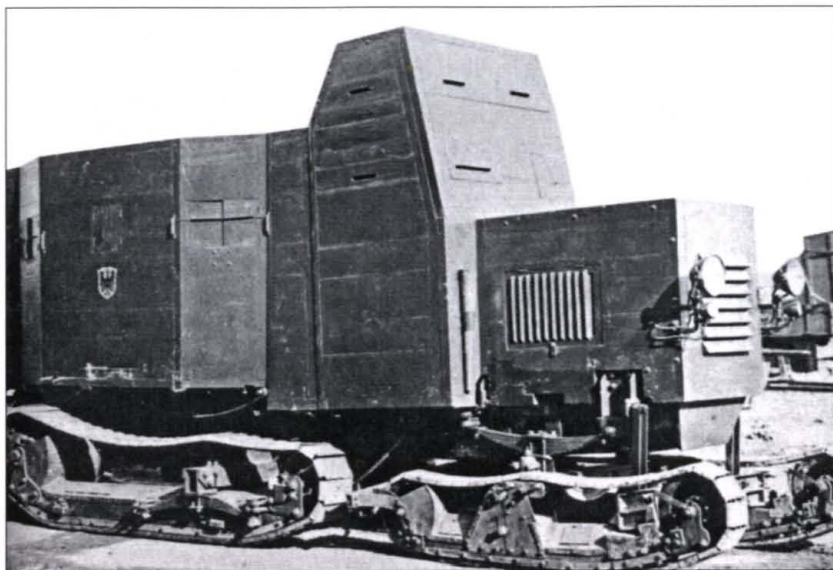
The first serious German effort to develop an armored fighting vehicle was an armored version of the tracked Bremer-Marienwagen. Even with only a mocked-up wooden superstructure, it proved to be hopeless in cross-country travel. (Patton Museum)
