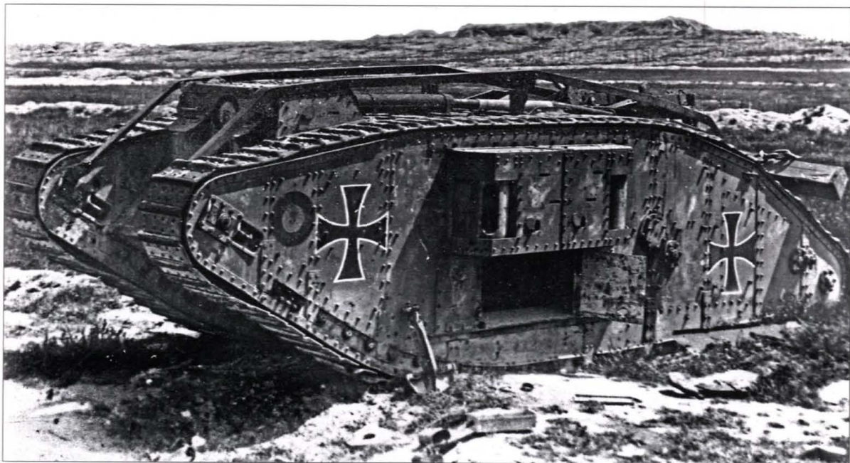
Another view of Panzer 107 Ännchen after it was abandoned near Fort de la Pompelle on June 1, 1918. (NARA)
