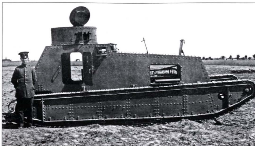
This single LK I light tank was constructed in 1918, but the armor was unacceptably thin. Plans were underway in the fall of 1918 to build the improved LK II but the war ended before any were ready for army service. (Patton Museum)
