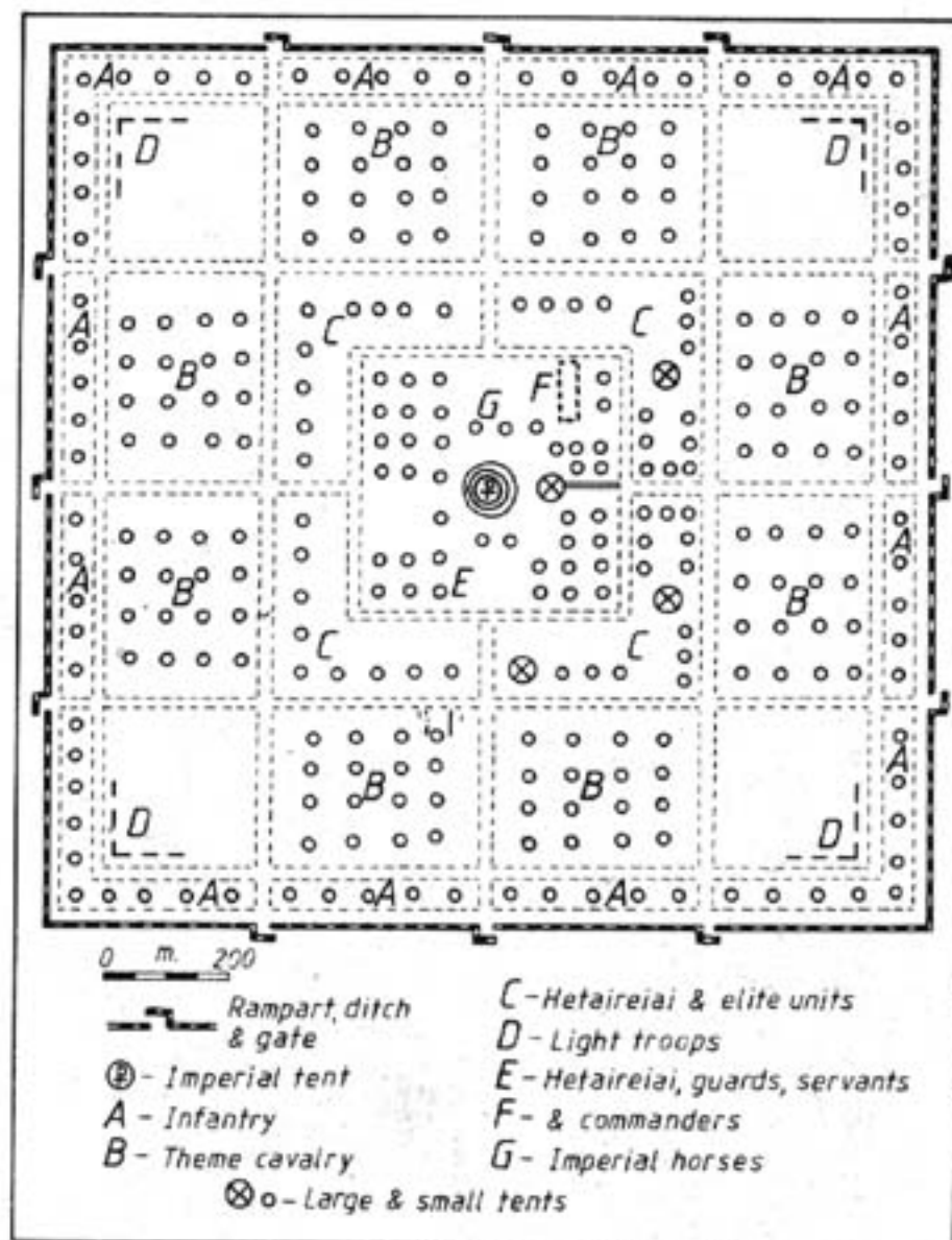
Ideal layout of an Expeditionary Camp, from a 10th century Byzantine treatise on organization and tactics (after Dennis).
