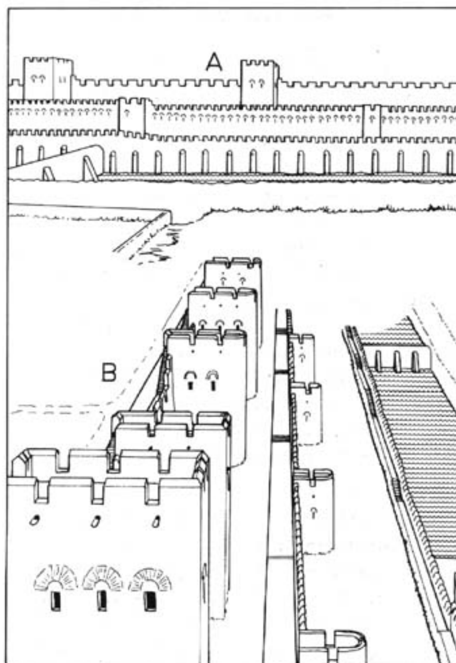
Reconstructed views of the land walls of Constantinople. (A) from outside the city; (B) looking south (after Meyer-Plath & Schneider).
