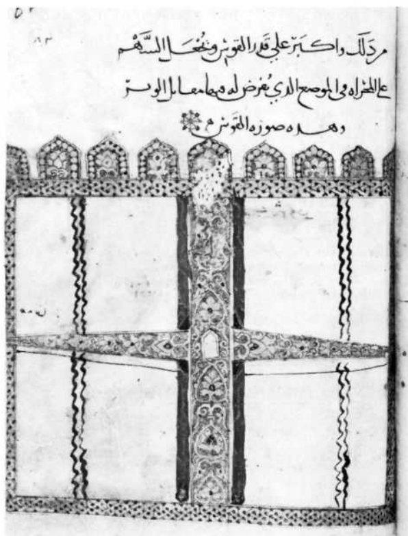
The ziyar and its loading mechanism. This was a large mounted crossbow reinforced by a wooden frame with taut ropes giving added strength to the arms of the bow. The bolt emerged from a small 'gateway' in the centre of the weapon. From al Tarsusi's late 12th-century military treatise (Ms. Hunt. 264, Bodleian Lib., Oxford) See Plate C1.
