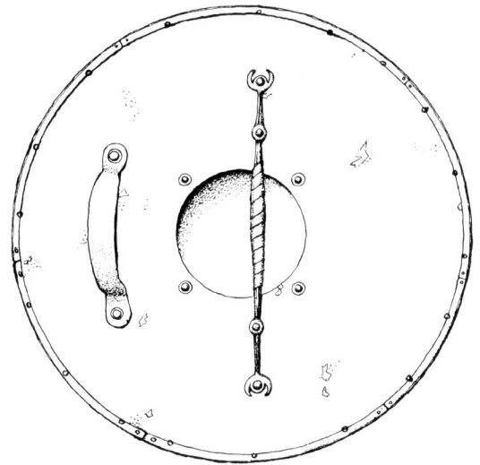
Reconstruction of the inside of an Anglo-Saxon shield, showing forearm strap and hand-grip.
