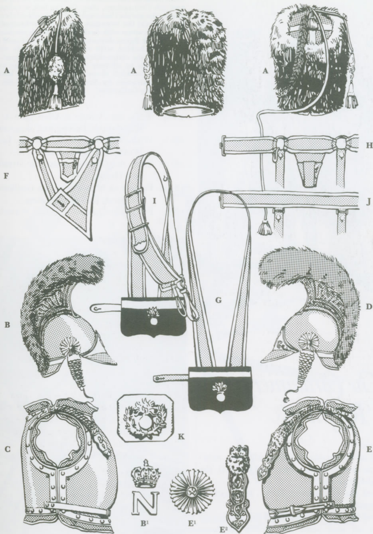
Equipment of carabinier officers and troopers: A : The carabiniers' bearskin as described by the 'AnX' Regulations, originally 318mm. but rarely below 350mm. towards 1810. B & B 1 : Helmet and front decoration as worn by troopers from late 1810. C : The troopers'-pattern cuirass. D : The officers' model of post 1810 helmet. Note that the crest is rather larger than that of the troopers' version. E , E 1 and E 2 : The officers' model cuirass, sunburst device from its breast and shoulder-strap detail. F : The 'AnIX'-pattern troopers' swordbelt. G : The troopers' cartridge-pouch prior to 1810. H : Troopers' swordbelt and bayonet frog, post 1809. I : Troopers' cartridge-pouch and musketoon crossbelt as carried post 1811. J : Officers'-pattern swordbelt, worn before and after 1810. K : Officers' swordbelt buckle
