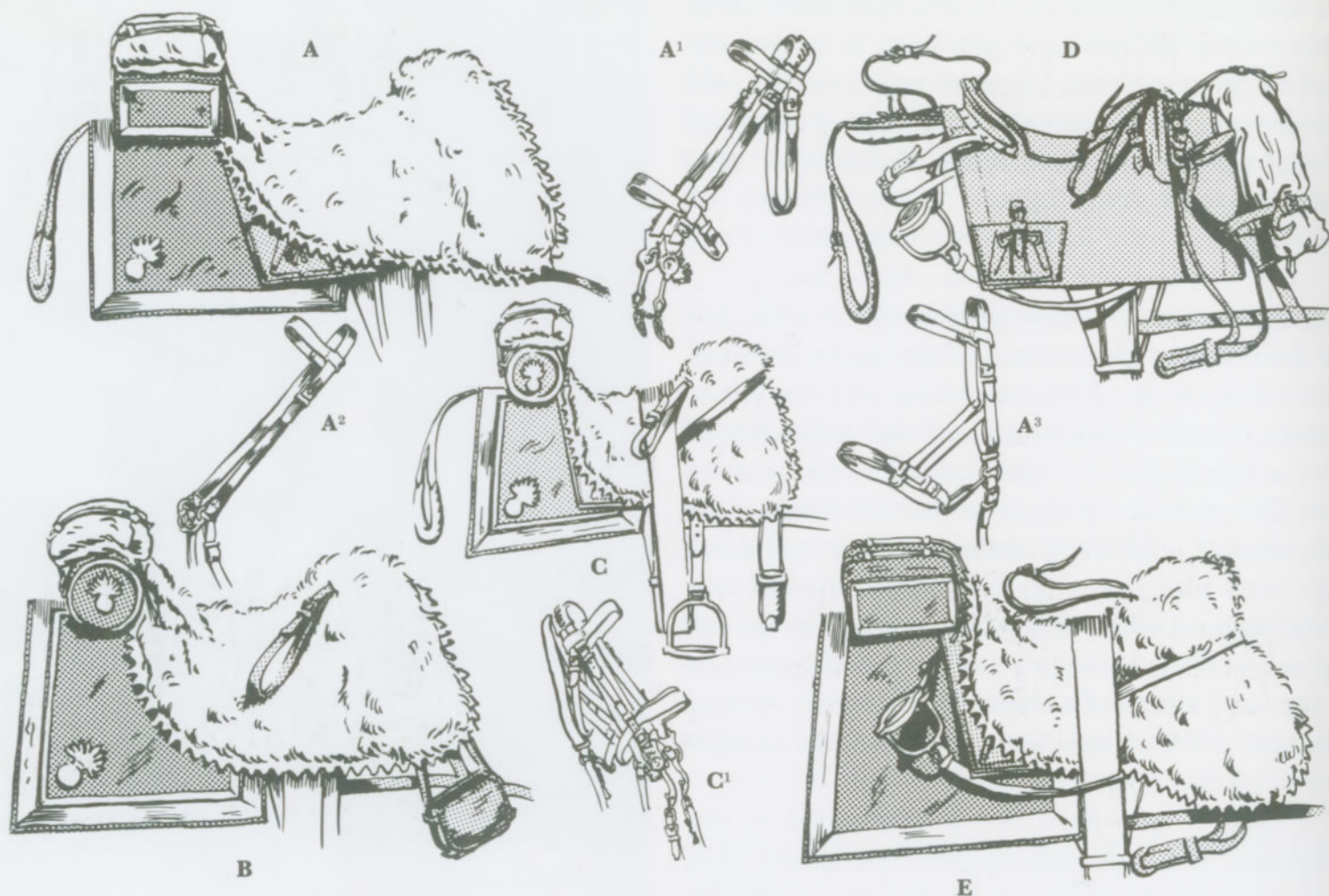
Saddles and harness of troopers of cuirassiers and carabiniers: A: Cuirassiers' saddle before 1812. The regimental number would be entered on the ends of the portemanteau in white. A 1 ; A 2 & A 3 : Headstall of the bridle, stable halter and parade halter of cuirassiers. B: Carabiniers' saddle before 1810. C: The carabiniers' saddle after 1810. C 1 : Carabiniers bridle, post 1810. D: Basic saddle, after Bardin, 1812. E: The same saddle but dressed for cuirassiers after the 1812 Regulations
