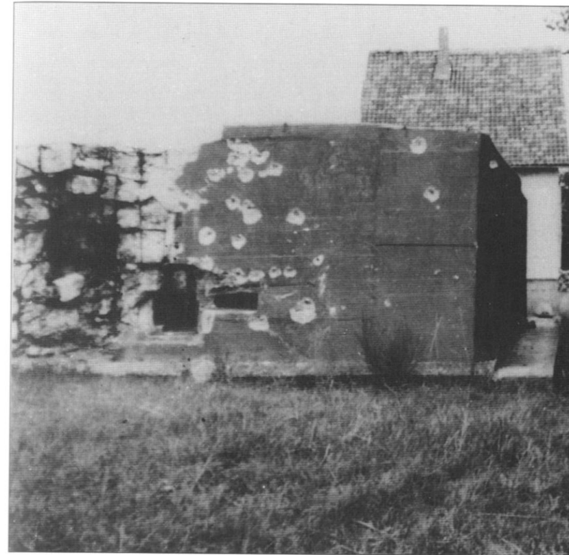
This bunker at Steckenborn sustained a massive hit just to the side of the aperture which penetrated the two metre thick reinforced concrete wall. American tank and SPG crews were instructed to target the doors and machine gun apertures which were recognised as being the weakest part of the structure. (Public Record Office)
