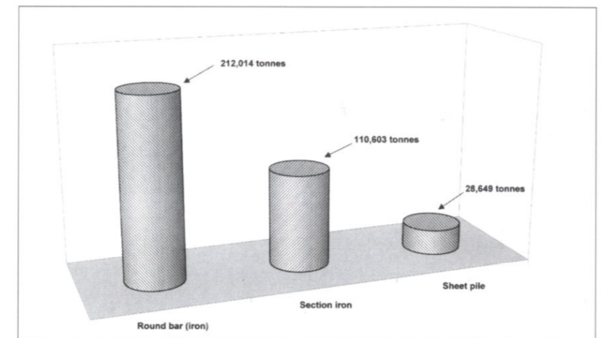
The round iron bar, section iron and sheet pile iron used in the construction of the West Wall in the period to 28 November 1938 (Army and Luftwaffe).
