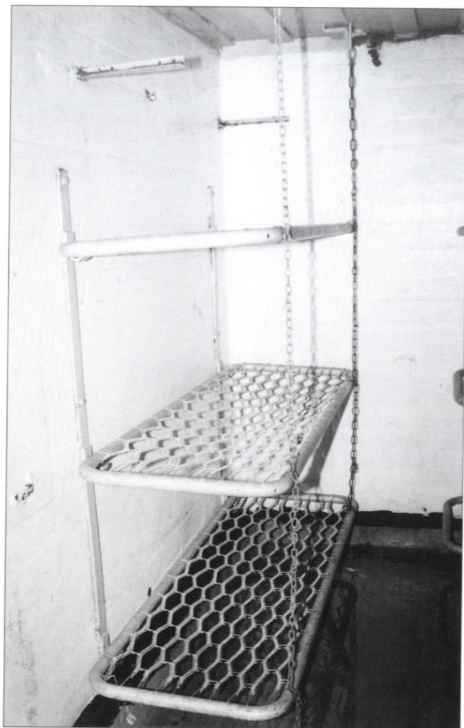
ABOVE The crew of the West Wall bunkers were afforded few luxuries, but most shelters were fitted with beds. The three tiered bunk beds were suspended on one side by chains fixed to the ceiling and on the other by hinges so that they could be folded against the wall when not in use. The steel framework was fitted with a wire mesh over which was stretched a sailcloth. A mattress and pillow were also provided. (Author's collection)
