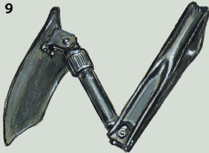
(9) The M1967 collapsible intrenching tool or "tri-fold e-tool." Lighter than earlier models, it was therefore less effective for digging in hard soil, and hacking with the blade locked at 90 degrees was less comfortable.
