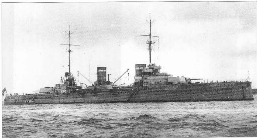
The first German battle cruiser set the pattern for the rest. The Von der Tann carried 11-in. (280 mm) guns compared to the 12-in. (305 mm) guns of the British Invincible class, but her main armour belt was 10-in. (254 mm) thick compared to 6-in. (150 mm). The first German capital ship to be powered by turbines, she could make 29 knots. (IWM)
