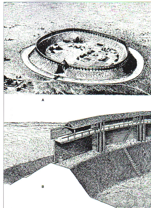
RIGHT A: Reconstruction of a typical fortified Russian outpost in the 12th/early 13th century. B: Reconstruction of a section through a typical Russian earth and timber fortification of the 11th-12th century.
