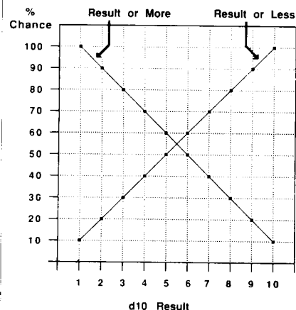
Probability Graph 3 d10
