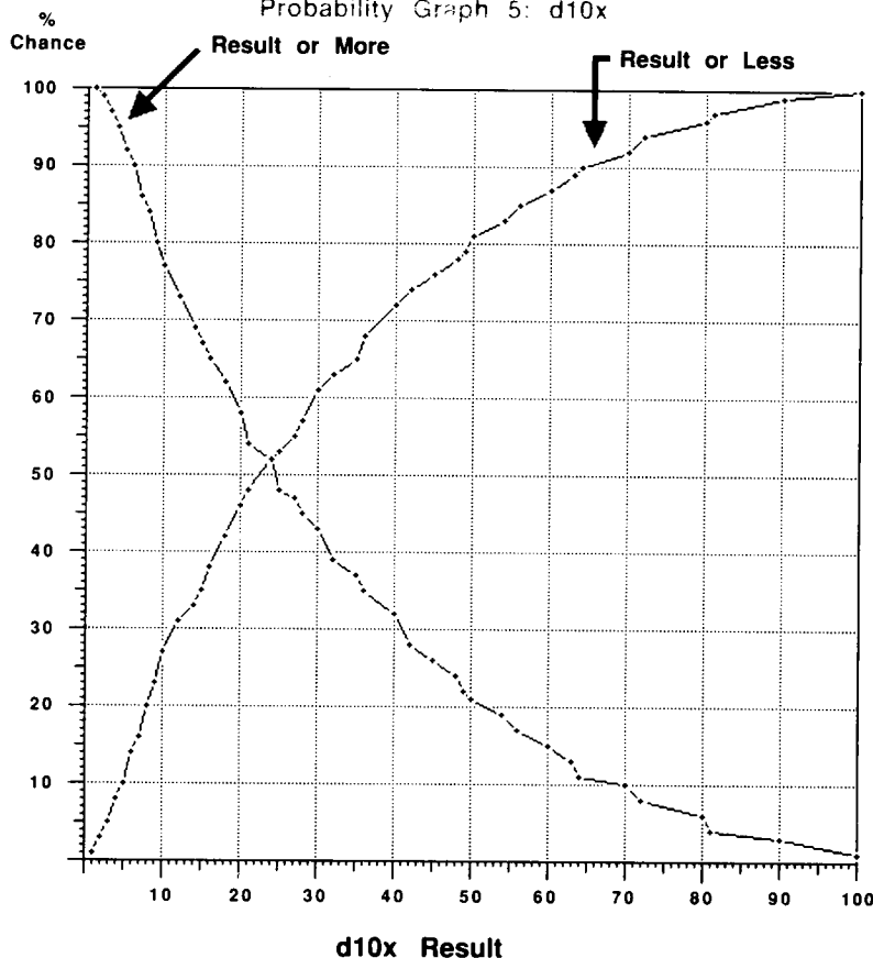
Probability Graph 5: d10x
