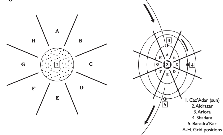
Figure 1: Sun and Moon Phase Grid Illustration
