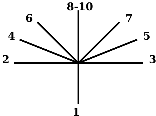
Figure 8.2: Scatter Diagram
