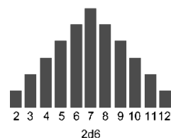
Illustration of 2d6 Bell Curve
