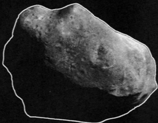
Stony Asteroid
