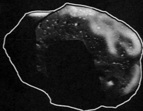
Carbonaceous Asteroid
