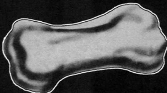
Metallic Asteroid
