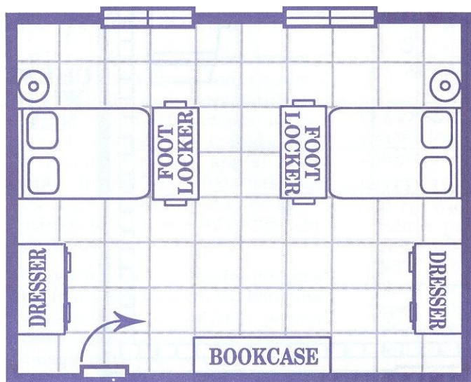
BEDROOM 40 (25' x 20')
