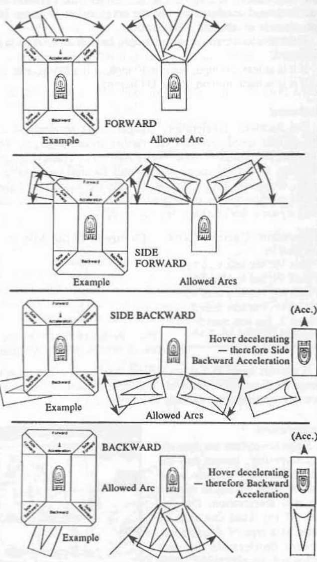
Figure 20 — Hovercraft Acceleration
