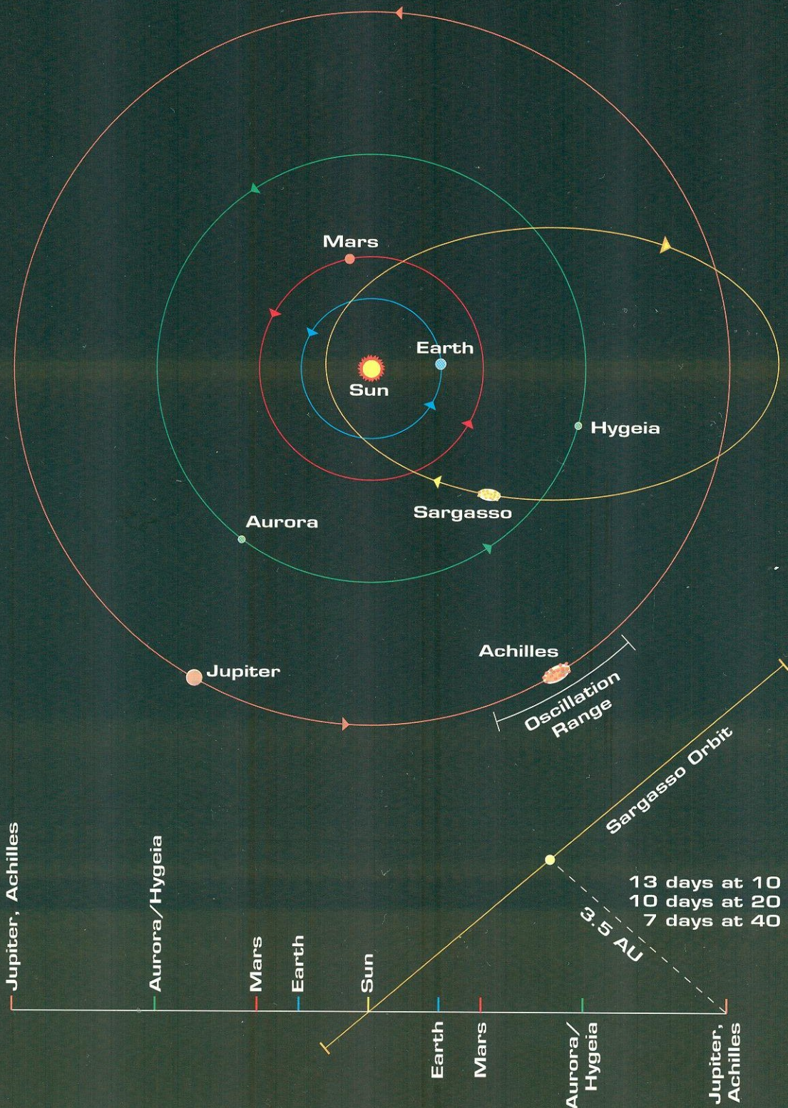
Side View Showing the Tipped Orbit of Sargasso
