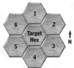
SCATTER DIAGRAM
